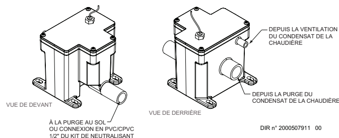
Figure 10-1 Siphon du condensat
