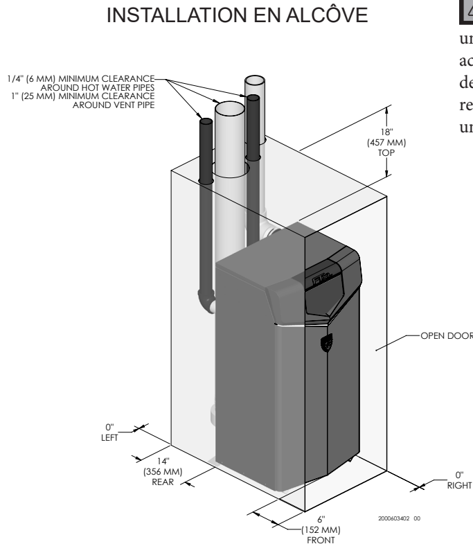
Figure 1-2 Installation en alcôve – Espaces minimum requis
